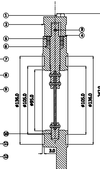
Section SS
